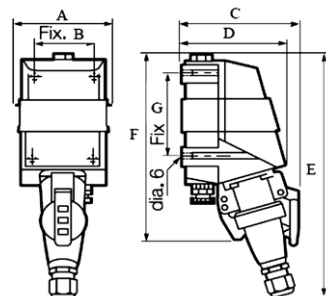
Wall mounting Socket
